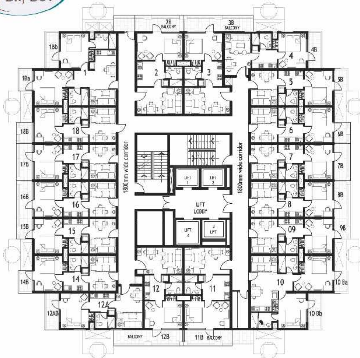
TENTATIVE TYPICAL FLOOR PLAN SERVICE APARTMENT
